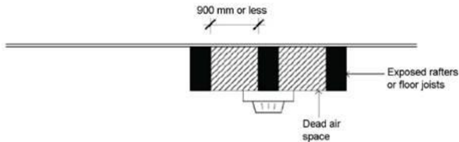
(e) Exposed rafters or floor joists
