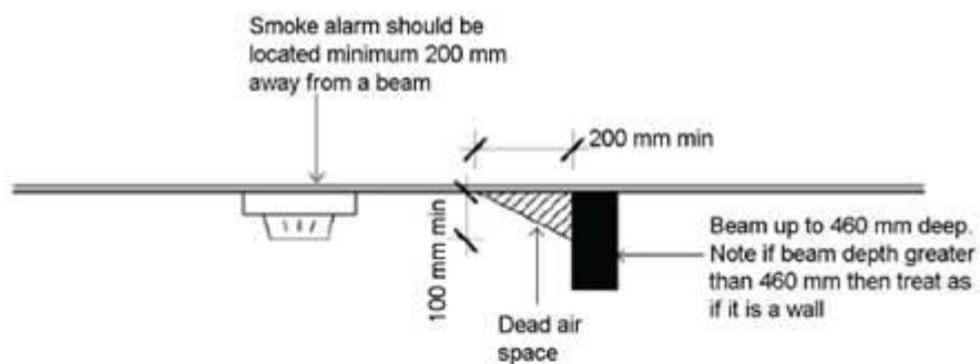
(d) Exposed beams (or other ceiling obstructions)
